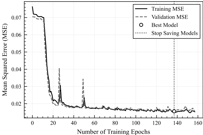
Learning Curve of LSTM Model for SolarPlant-3 (Gyeongju)
